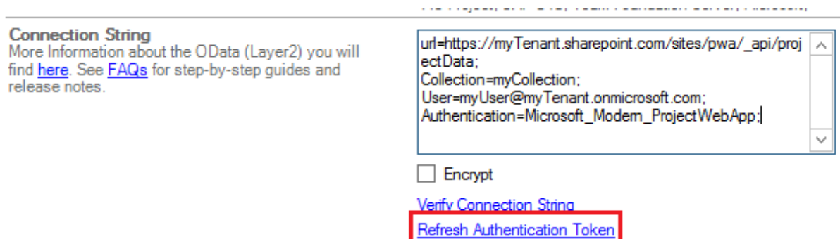
Figure 86 – Link in the UI to refresh the authentication token for Microsoft_Modern_Dynamics_ERP authentication
